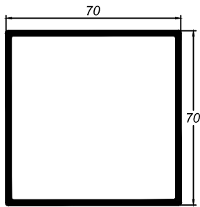
REF2001 (e=2mm)
