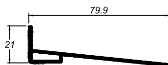
2019 BASE PINGADEIRA
