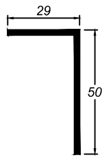
2046 CANTONEIRA 50 X 29
