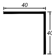
2047 CANTONEIRA 40 X 40
